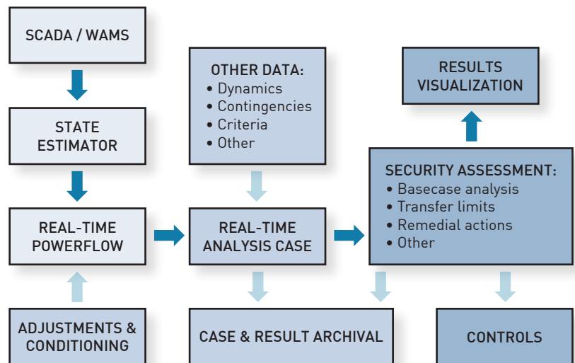
Online DSA flowchart
